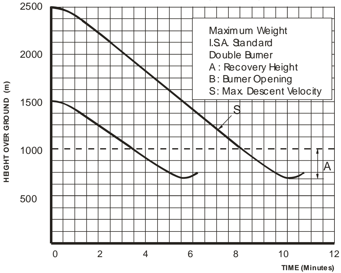
SIZE 180 (5100 m3)
