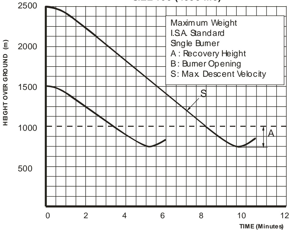
SIZE 160 (4550 m3)
