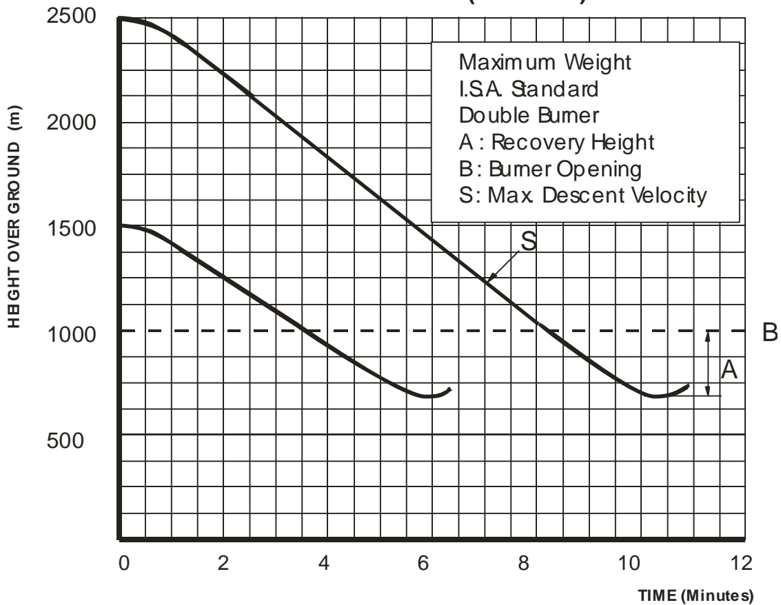
SIZE 210 (6000 m3)
