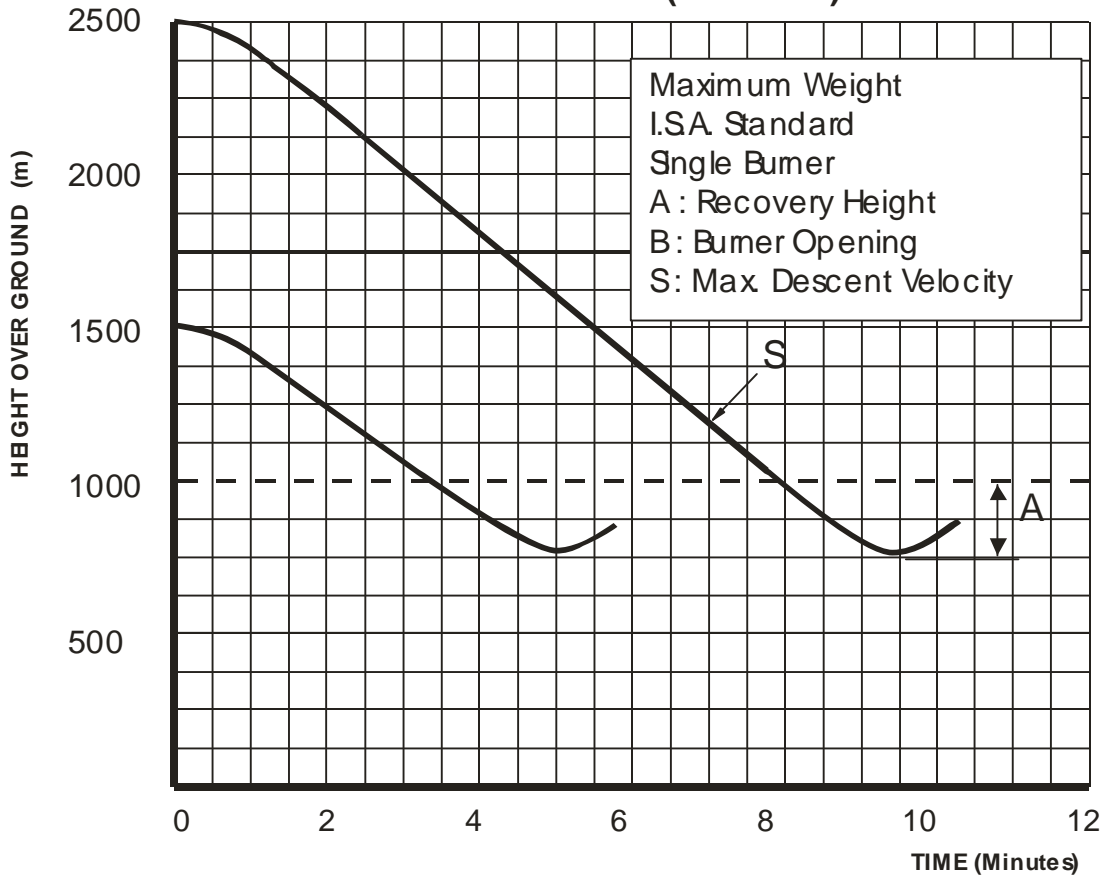
SIZE 150 (4245 m3)
